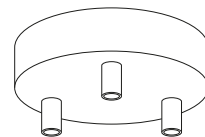
KRM573FVNTERM 3 HOLE Ø 120MM H 25MM
