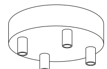
KRM574FV0TSTERM 4 HOLE Ø 120MM H 25MM
