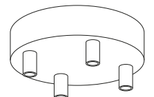
KRM574FRATERM 4 HOLE Ø 120MM H 25MM
